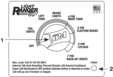
Fig. 2 - #9101-D20C Control and Information Panel
