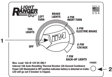
Fig. 2 - #9101-18C Control and Information Panel
