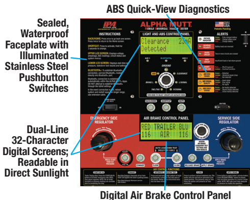
Digital Air Brake Control Panel
