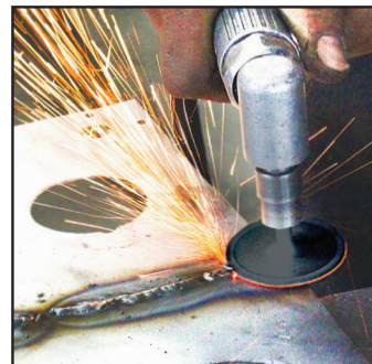
Grind, Cut and Undercut with One Wheel
