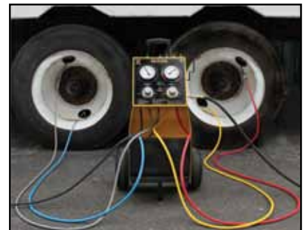
Inflate and equalize steer and drive tires simultaneously. #TEQ-5HLTC Lock-On Tire chucks are available separately.*
