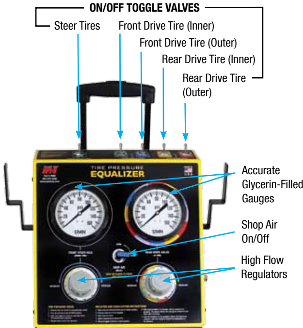
Inflate and equalize steer and drive tires simultaneously. #TEQ-5HLTC Lock-On Tire chucks are available separately.*
